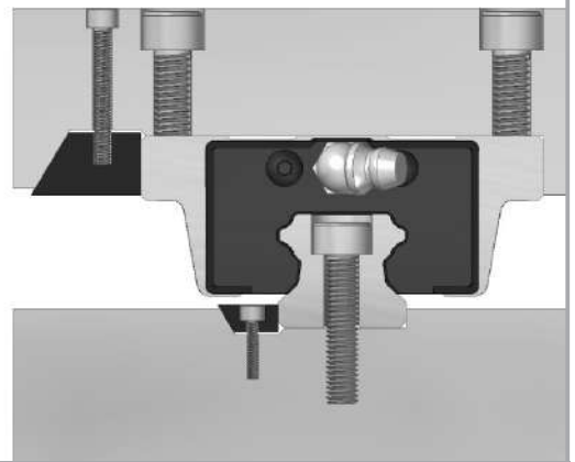
Figure 9. Pushing a tapered plate
