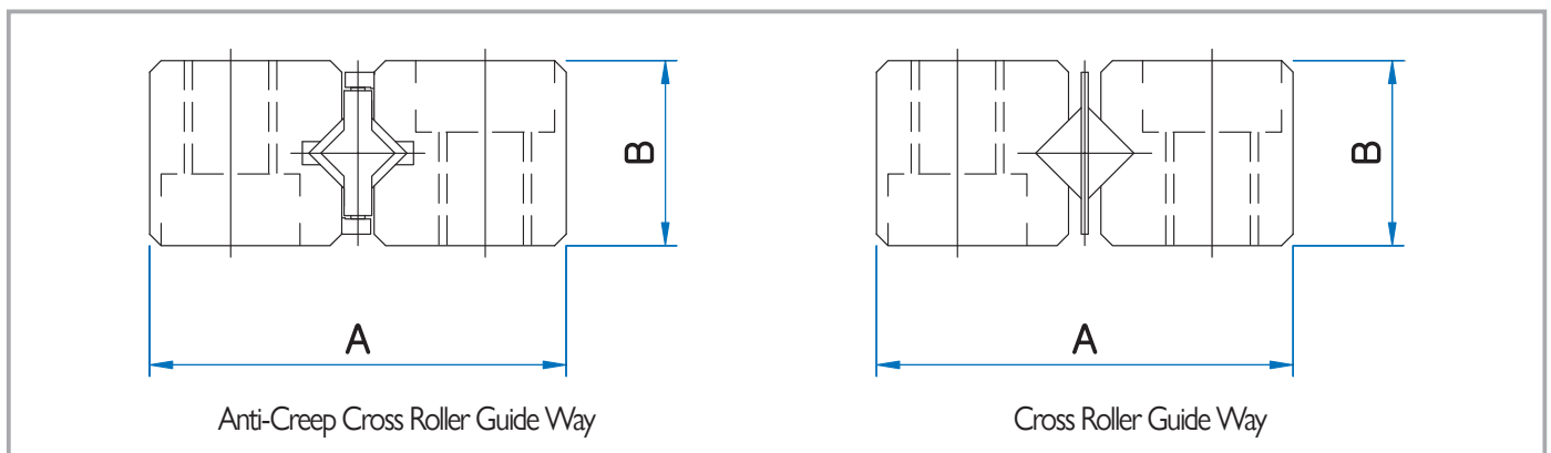
Figure 2. Dimensional compatibility
