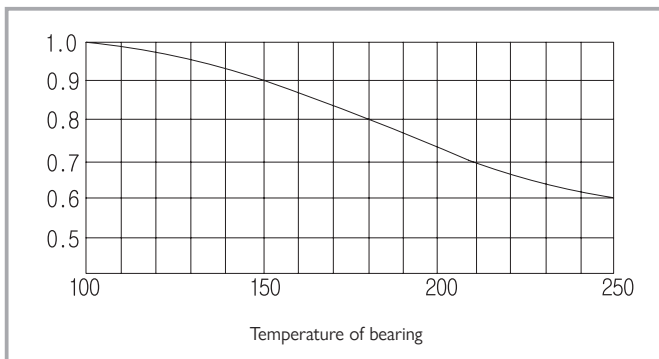
Figure 2. Temperature factor
